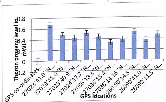
Fig3: Variation of thoron progeny level(RCC)
