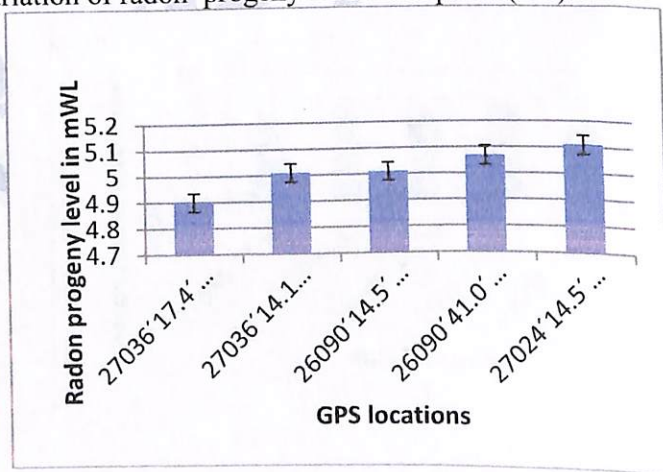
Fig2: Variation of radon progeny level with place (AT)
