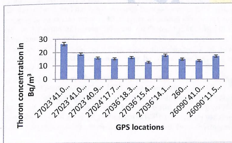
Fig 7: Variation of thoron concentration (RCC)
