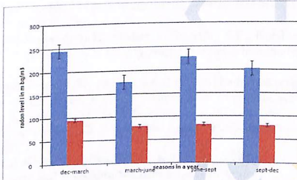
Fig3: Variation of radon concentration
