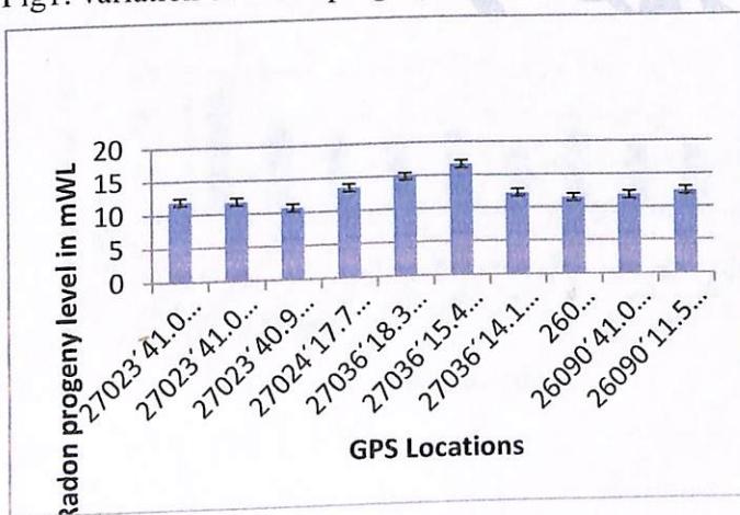
Fig1: variation of radon progeny level (RCC)
