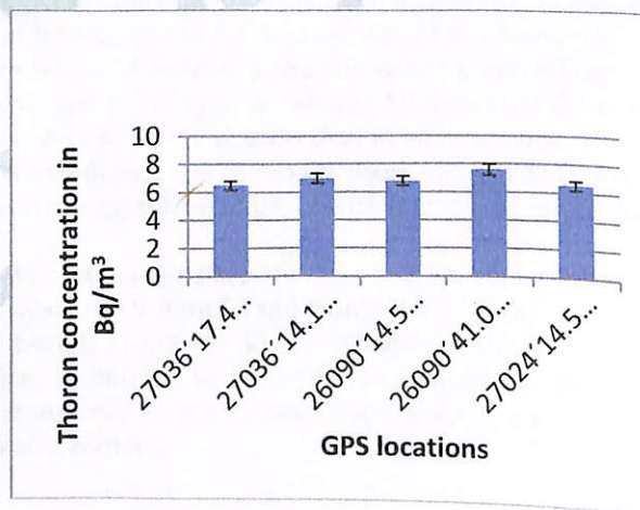
Fig8: Variation of thoron concentration(AT)
